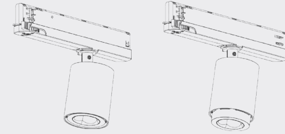
TRACK Ø 65 mm | max. 135 mm
